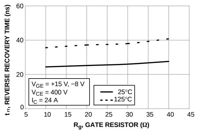
Figure 46. Typical Reverse Recovery Time vs. Rg
