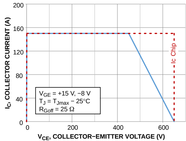
Figure 56. IGBT RBSOA
